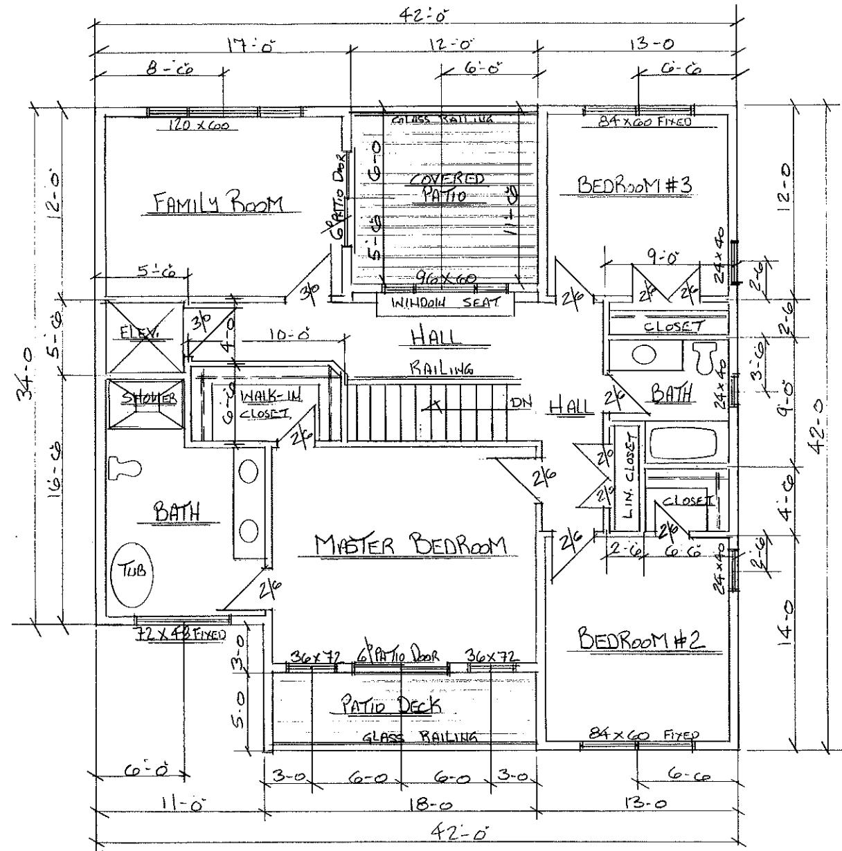
UPPER FLOOR PLAN (1456 SF) SCALE 1/4"=1'-0"
