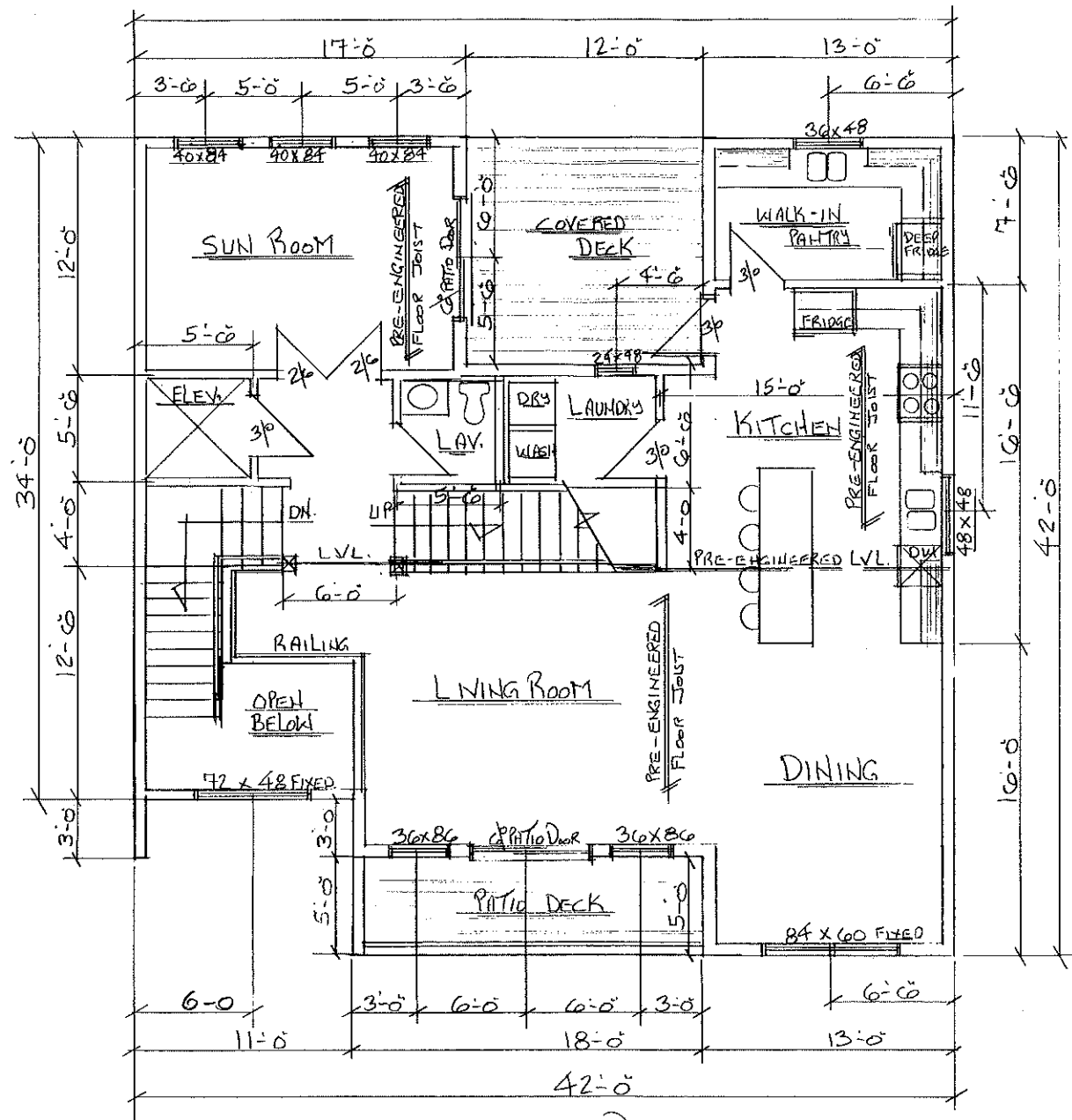
LOWER FLOOR PLAN 1456 SF SCALE 1/4"=1'-0"
